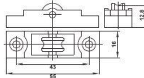
Single Roller With Groove PL50574A
