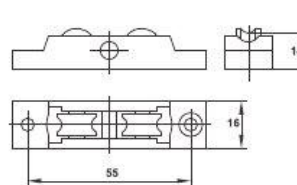
Double Roller With Groove PL50671A
