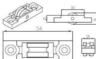
Single Roller With Groove PL50575
